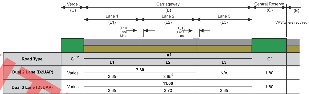
Dual Carriageway
