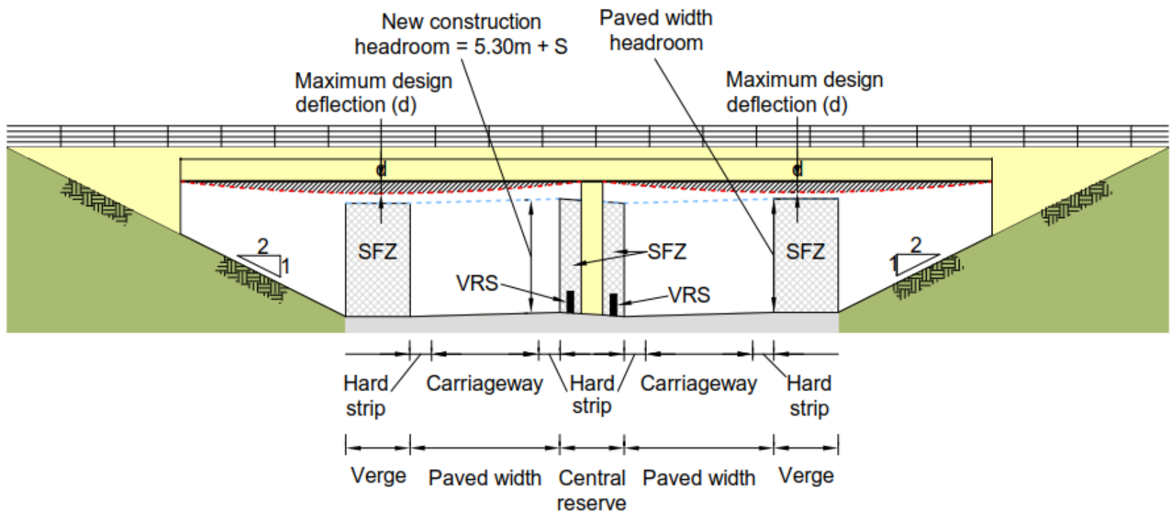
Figure 4.8b Headroom and SFZ for a 2 No. span structure crossing a dual carriageway
