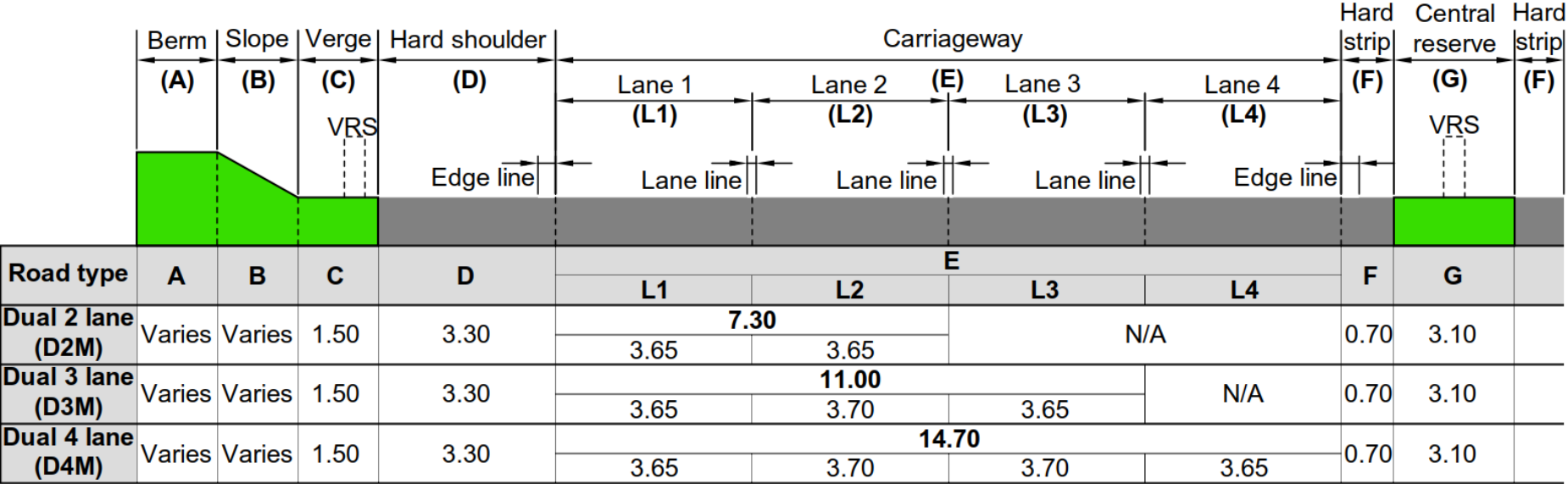
Figure 2.1.1N1a Dimensions of cross-section components for rural motorway mainline
