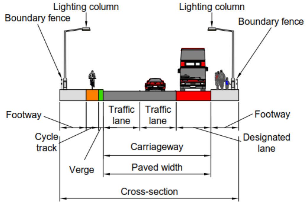
Typical urban single carriageway cross-section components
